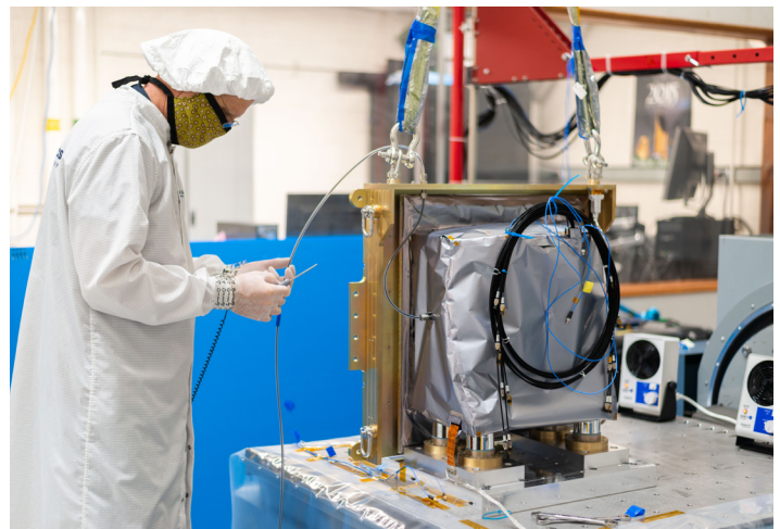
Assembled flight SDA being prepared for vibration testing.
