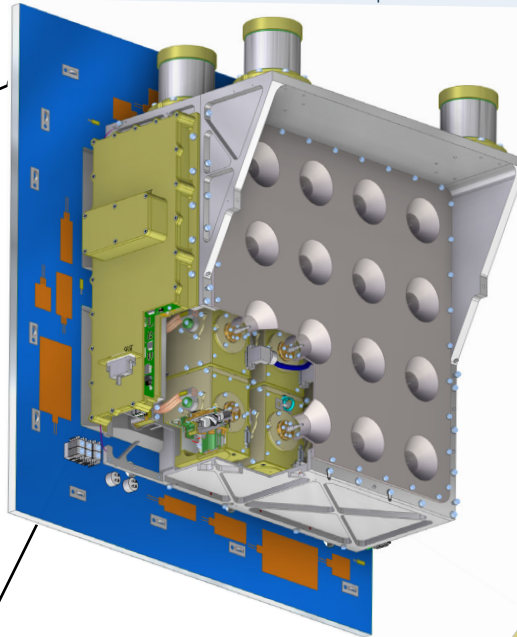
The SWIR SIDECAR Module (SSM) digitizes 32 analog channels and communicates with the spacecraft Data Acquisition Unit (DAU).
