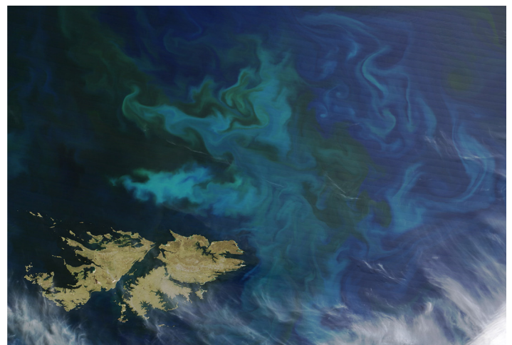
Phytoplankton blooms off the Falkland Islands. (Credit: NASA/Jeff Schmaltz, https://earthobservatory.nasa.gov/images/ )
